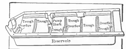
Fig. 4—Lower half of Thomas crankcase casting, illustrating disposal of splash troughs and overflow holes
